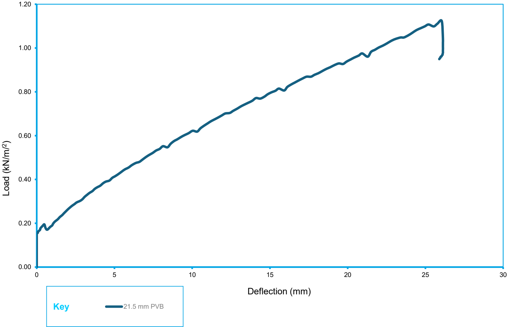
Chart 2 - Load Deflection Curve for Posi Base Balustrade System Base Mounted into Concrete when Subjected to a Uniformly Distributed Load
