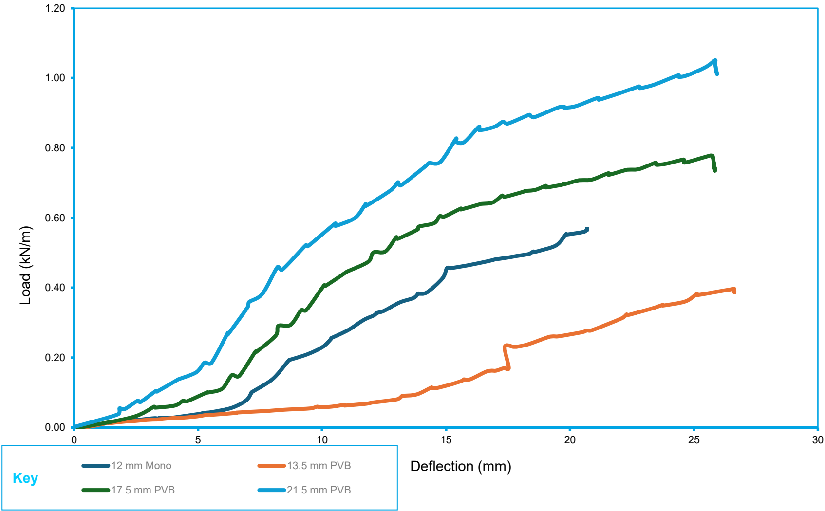
Chart 1 - Load Deflection Curve for Posi Base Balustrade System Base Mounted into Concrete when Subjected to a Horizontal Line Load
