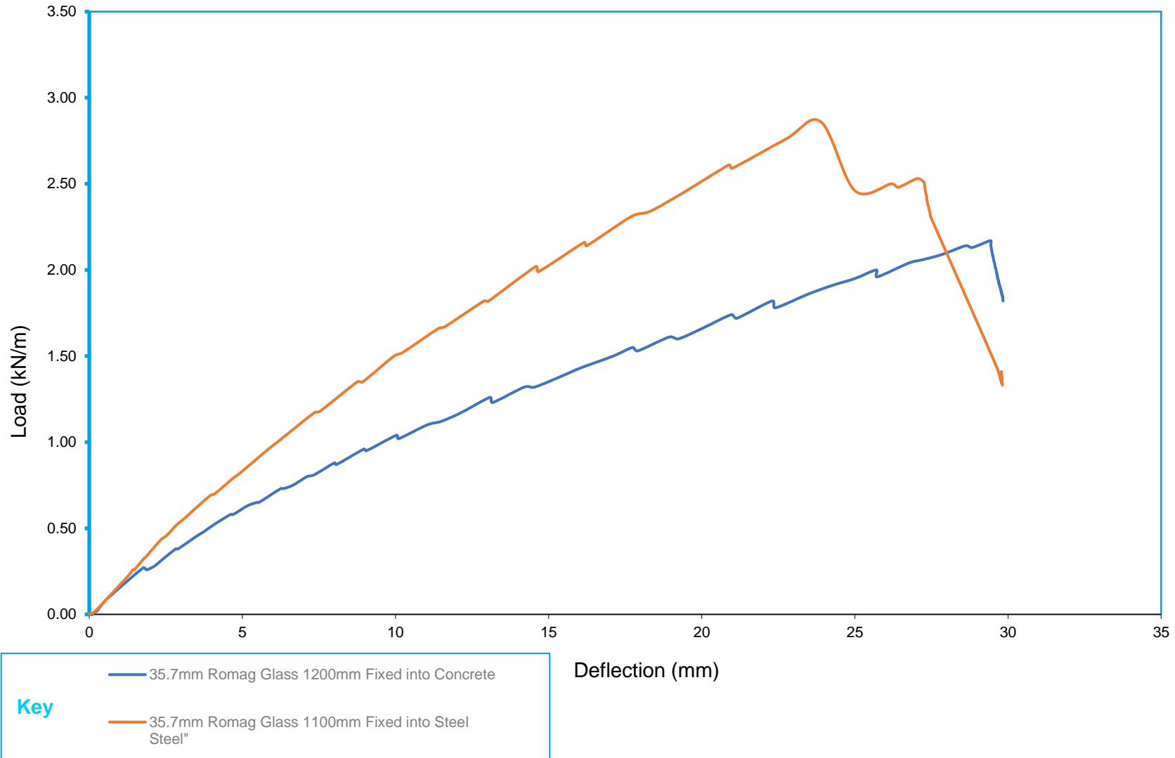
Chart 1 - Load Deflection Curve for Pure Vista MegaGrip System Incorporating 35.7 mm Romag Glass
