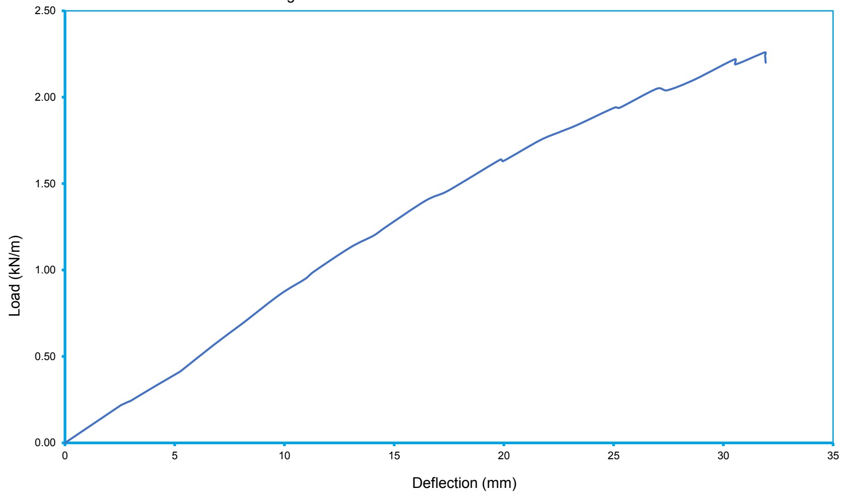
Chart 1 - Load Deflection Curve for Pure Vista MegaGrip System Incorporating 35.7 mm Romag Glass Fixed into Concrete
