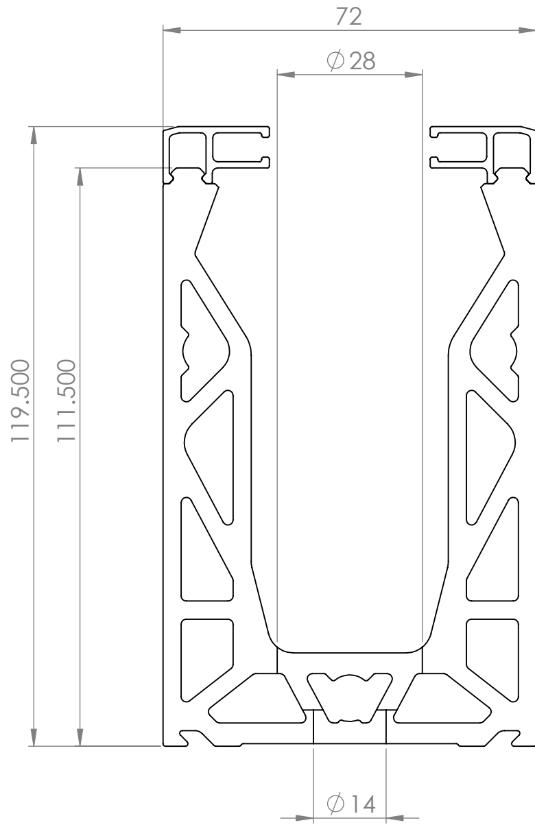
SECTION B-B SCALE 1 : 1
